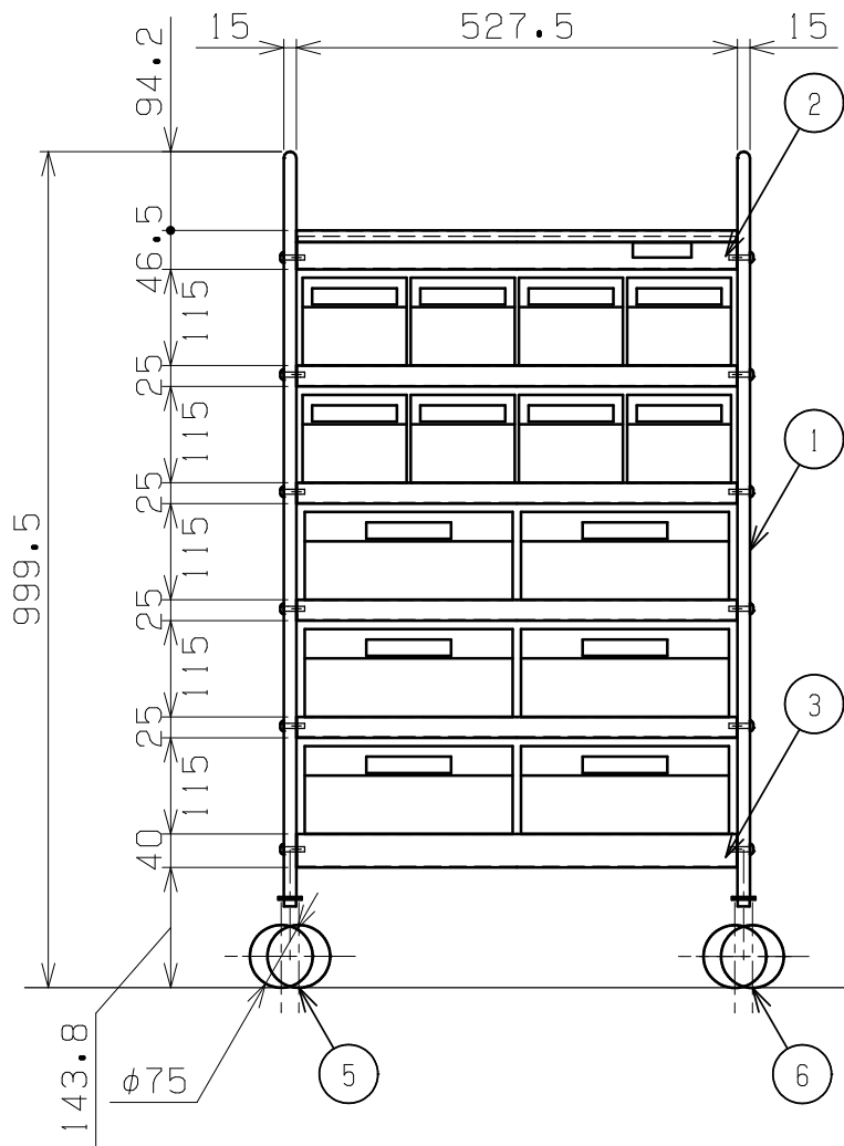
図示:CSD-86TWD
