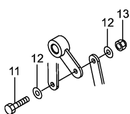
DETAIL "H"
