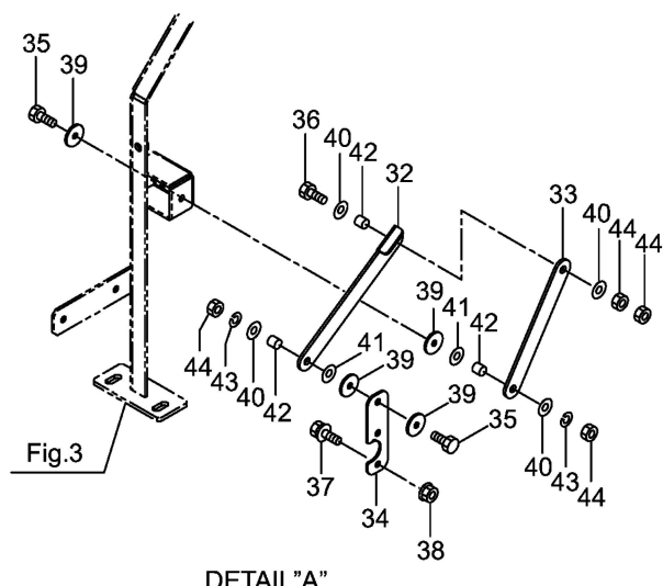
DETAIL "A"
