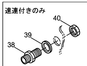
DETAIL "D"
