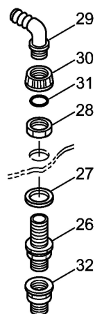
DETAIL "A"
