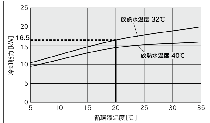
HRSHF200-W□-20/40-□
