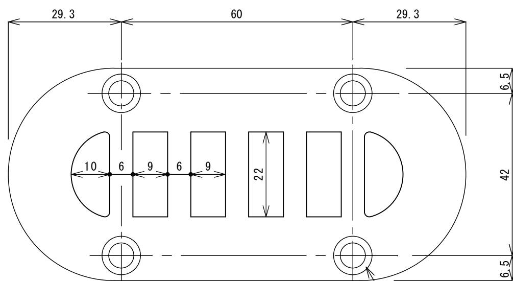
SUS目皿
