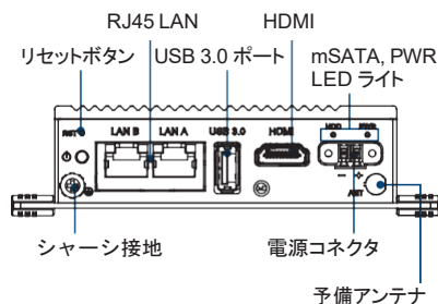
UNO-2271G-E21BE/E021AE
