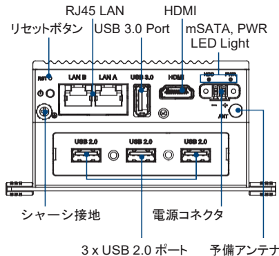
UNO-2271G-E22BE/E022AE
