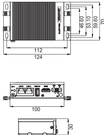
UNO-2271G-E21BE/E021AE
