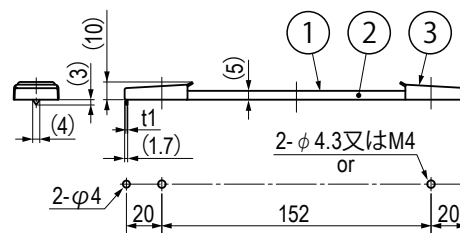
取付穴図 Holes for Installation
