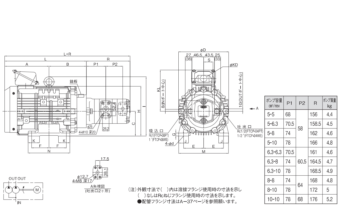
HBPG-3※4-TCP22-※-※R-B
