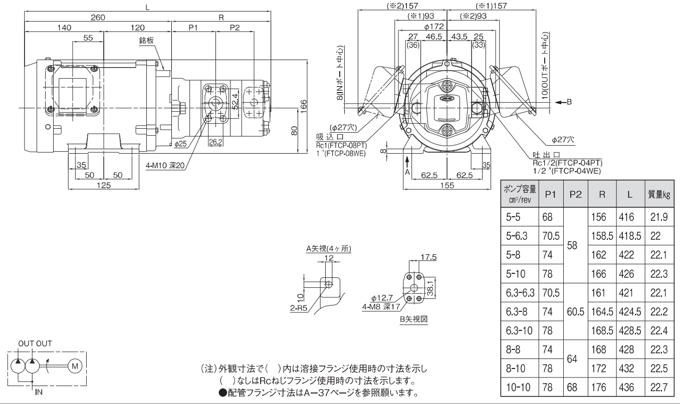
HBPG-3BH4※-TCP22-※-※R-B
