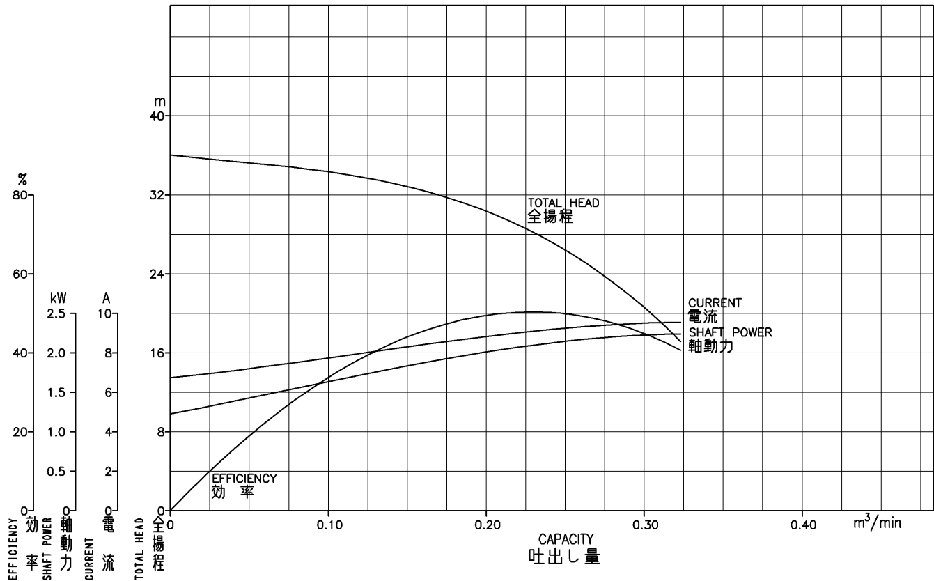
予想性能曲線図 PUMP PERFORMANCE CURVES
