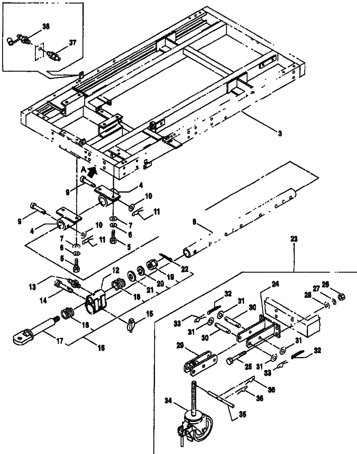
DETAIL - A
