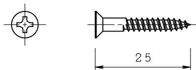
皿木ネジ 3.5 × 2.5
