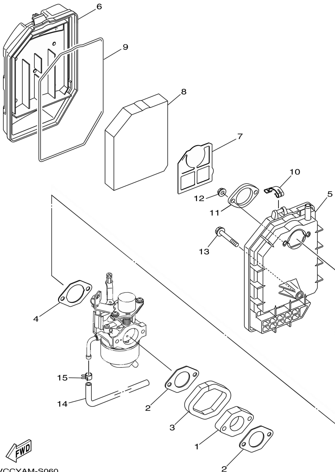
FIG. 6 INTAKE
