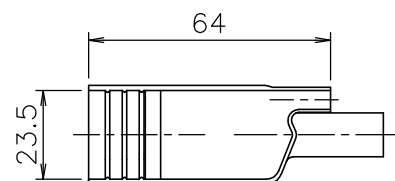
断面F-F
