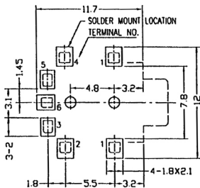
PCB HOLE & SURFACE MOUNT LAYOUT
