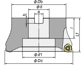
Fig.3 (エア穴無し) Without air hole
