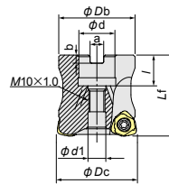
Fig.1 (エア穴付き) With air hole
