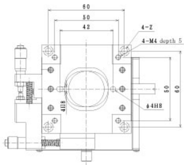
Bottom surface
