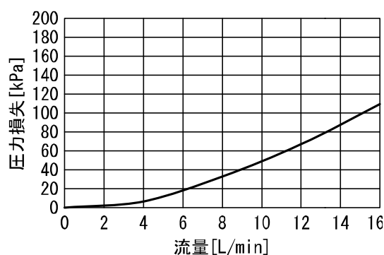
FC3W520-□
