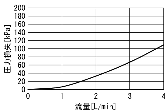
FC3W504-□
